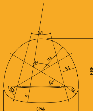
Standard Underpass UC
