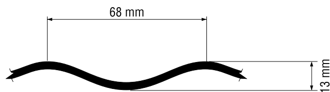
Fig. 1 - Typical corrugation (MP68)
