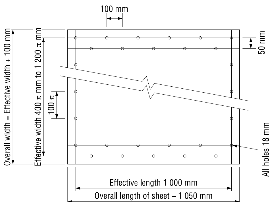
Fig. 2 - Typical plate
