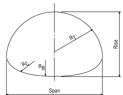
Fig. 5 - Pipe Arch
