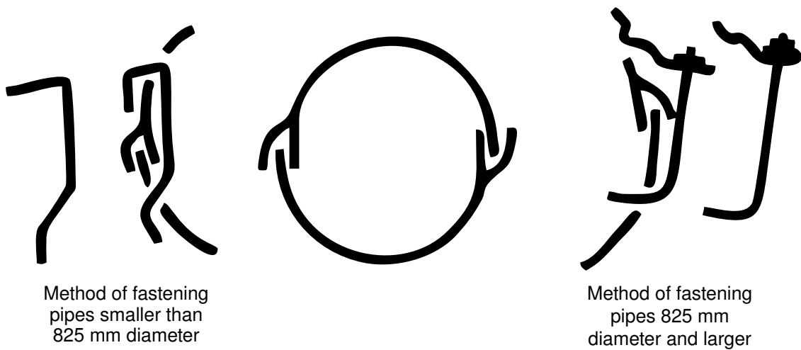
Fig. 4 - Fastening method
