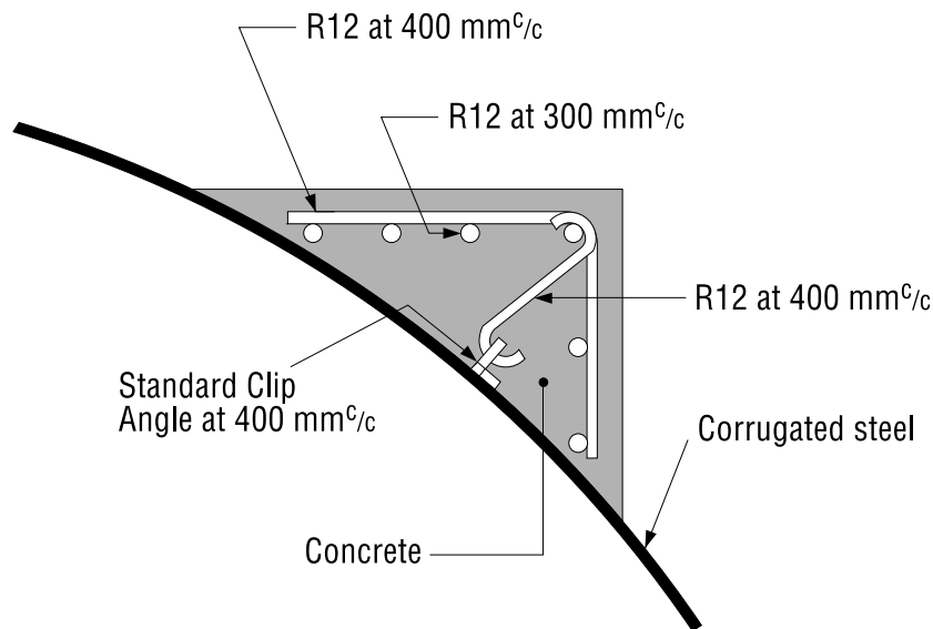
Fig. 8 - Typical thrust beam detail
