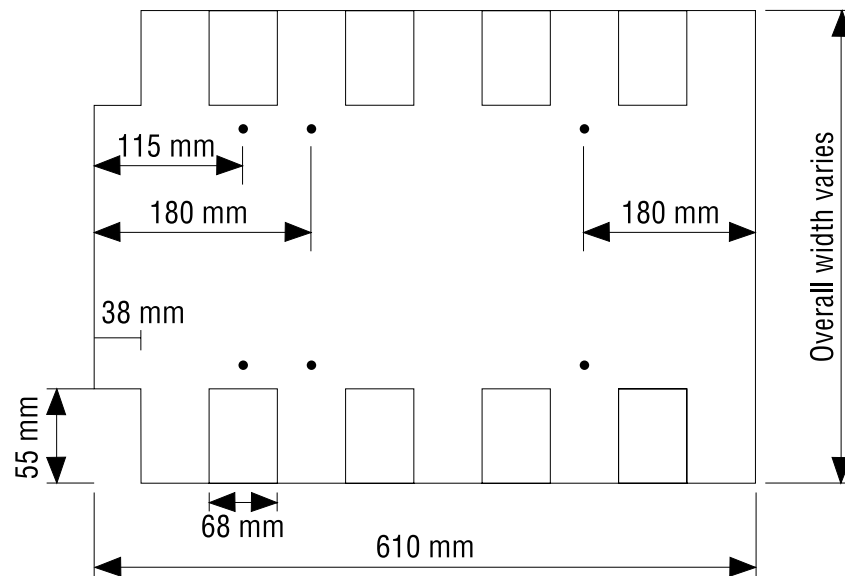
Fig. 2 - Typical plate
