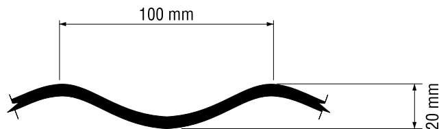
Fig. 1 - Typical corrugation (MP100)
