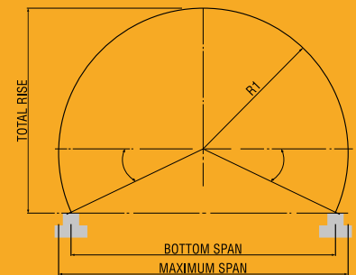
High Profile Underpass UA
